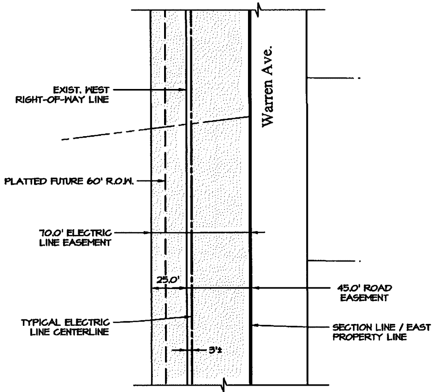
EASEMENT DETAIL SCALE: 1" = 50'
