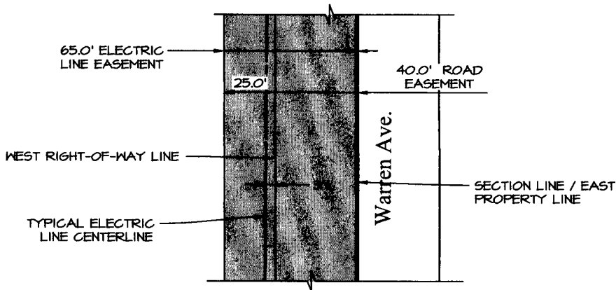
EASEMENT DETAIL SCALE: 1" = 50'
